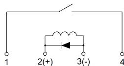
[Wiring diagram]
