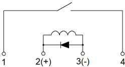
[Wiring diagram]
