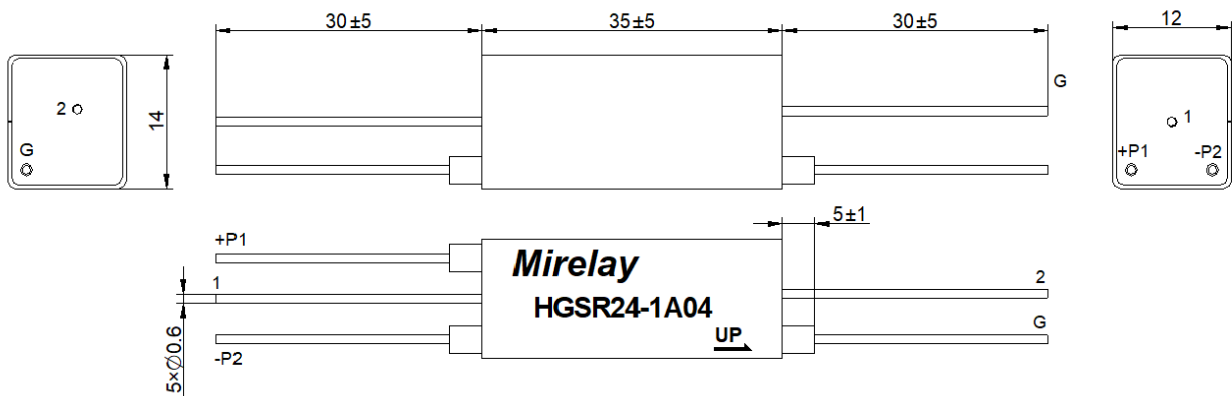
[Pin Layout]
