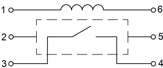
[Wiring diagram]
