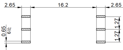
[MOUNTING PAD TOP VIEW]
