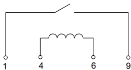
[Wiring diagram]
