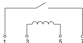
[Wiring diagram]
