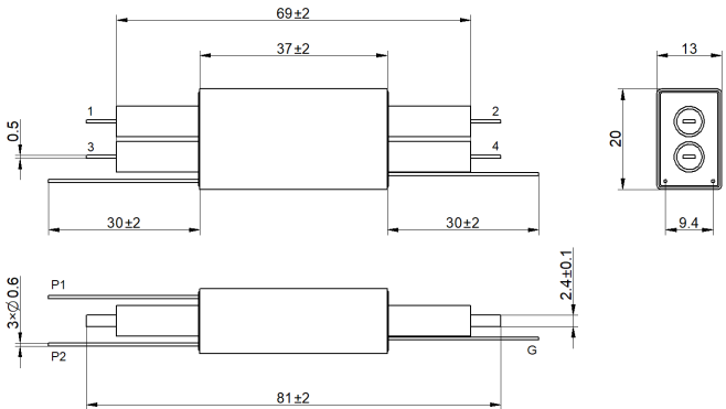
Layout[Top View]
