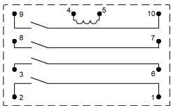
Layout[Top View]
