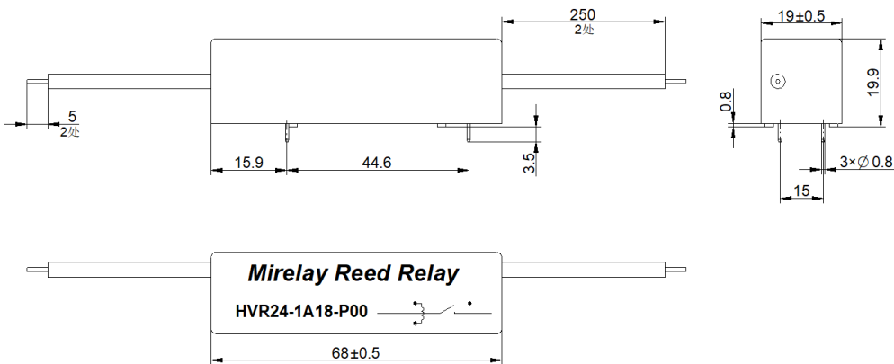
[Pin Layout]
