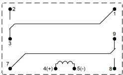
Layout[Top View]
