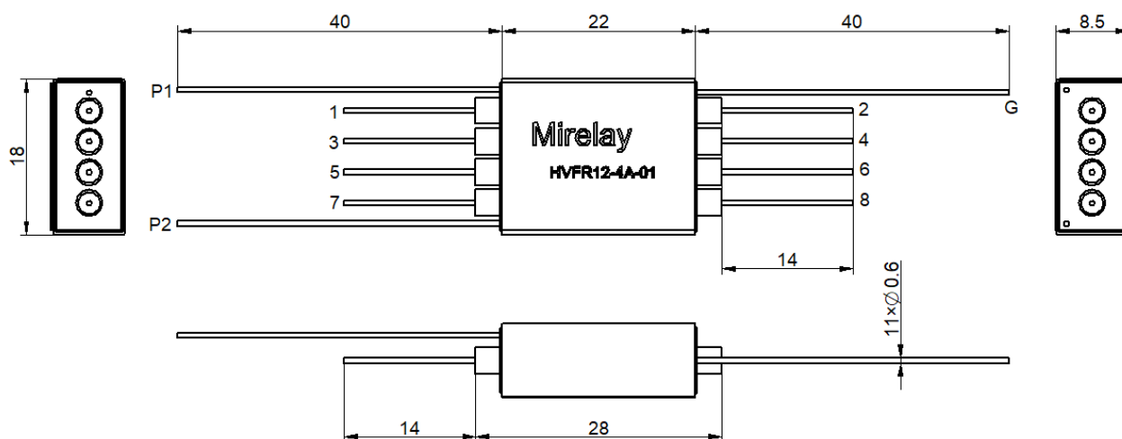
[Pin Layout]
