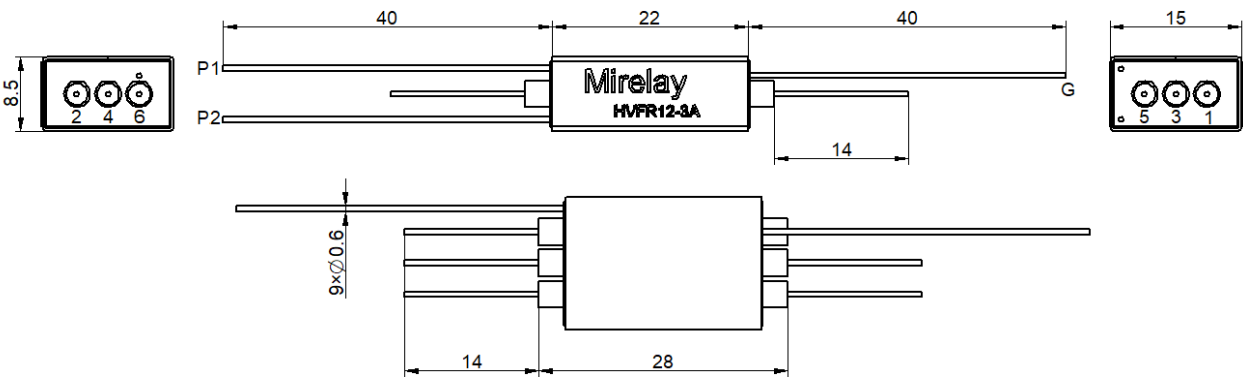
[Pin Layout]
