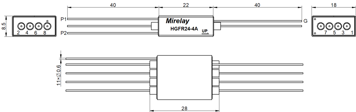
[Pin Layout]
