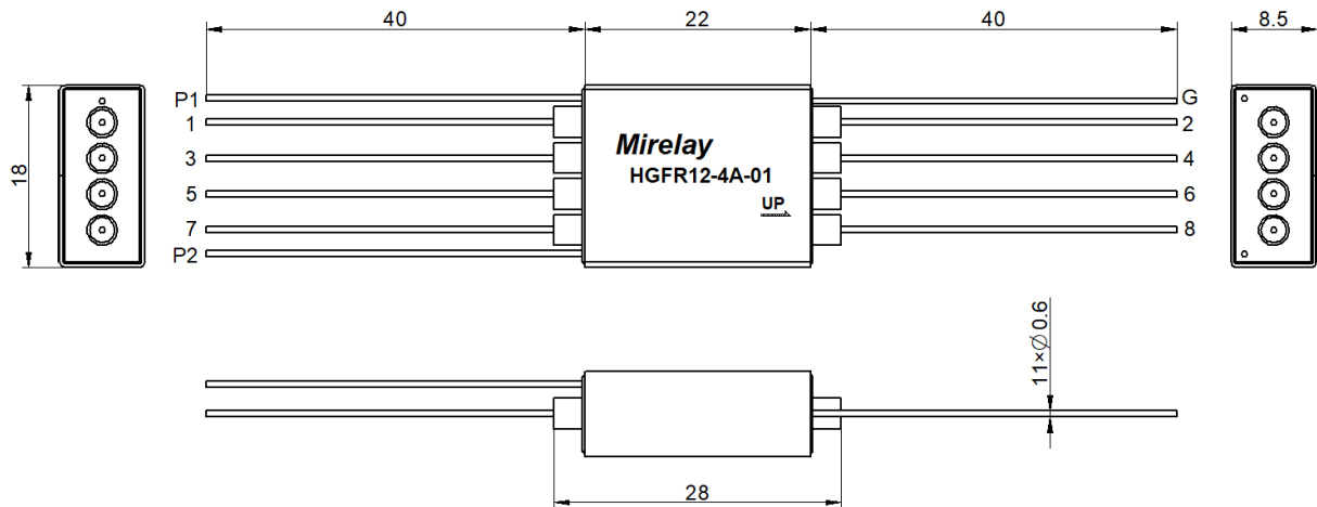
[Pin Layout]
