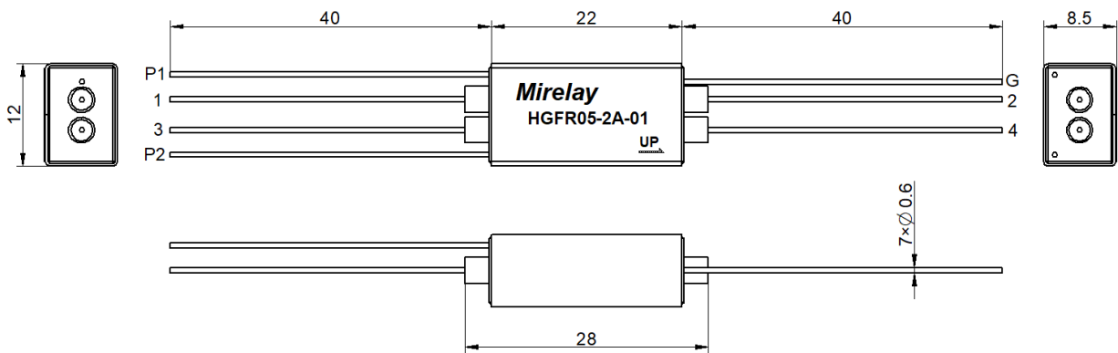
[Pin Layout]
