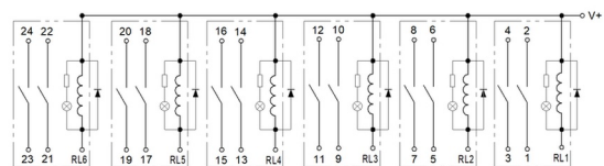
Source wiring diagram
