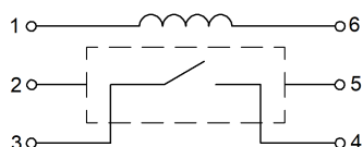
[Wiring diagram]
