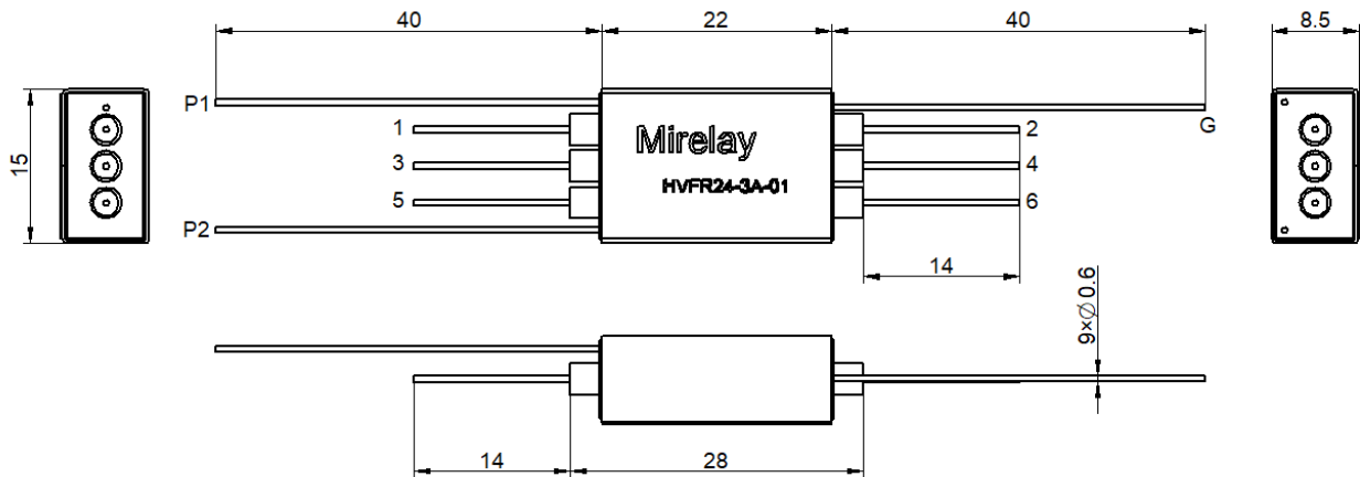
[Pin Layout]
