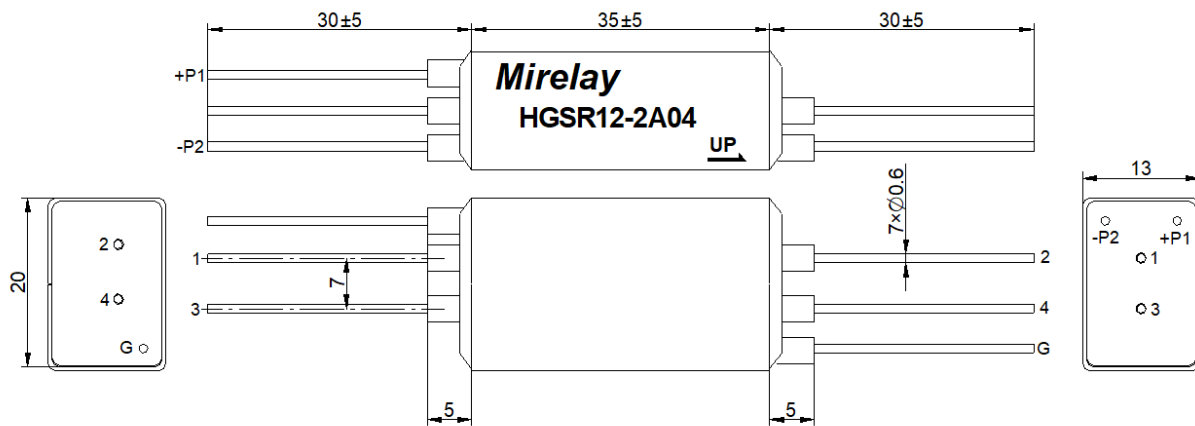
[Pin Layout]
