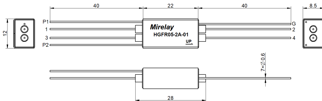
[Pin Layout]
