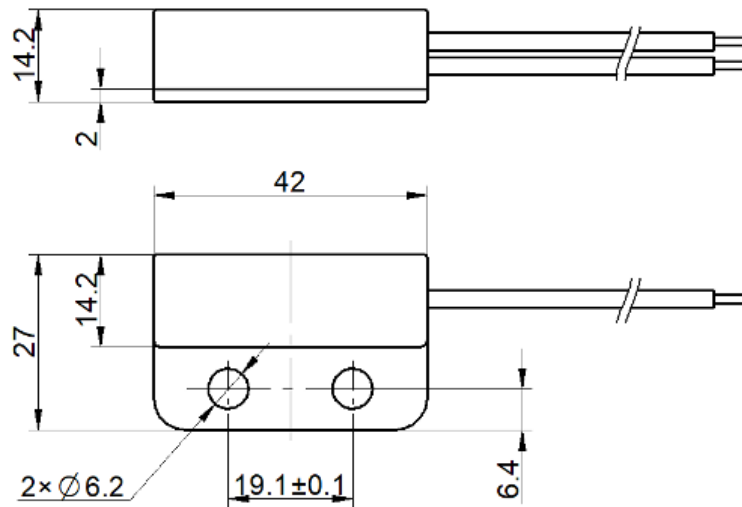
MRS18 Outline Drawing
