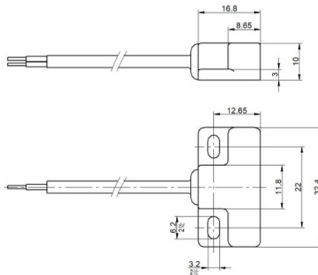
MRS16 Outline Drawing
