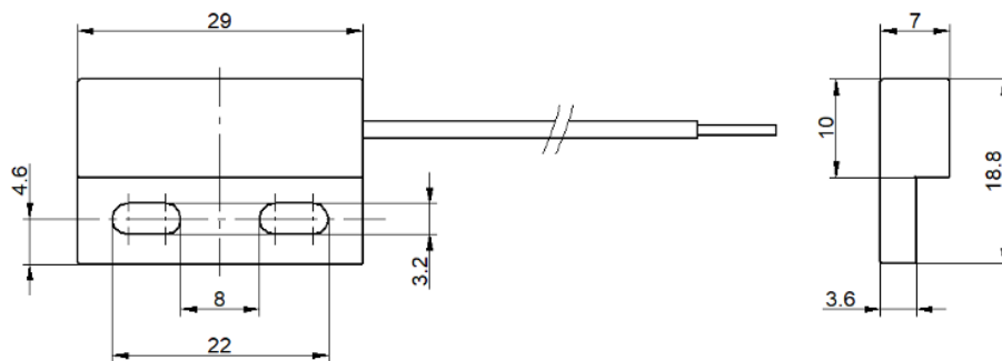
MRS12 Outline Drawing
