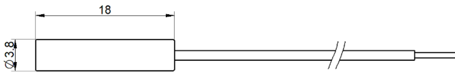
MRS11 Outline Drawing
