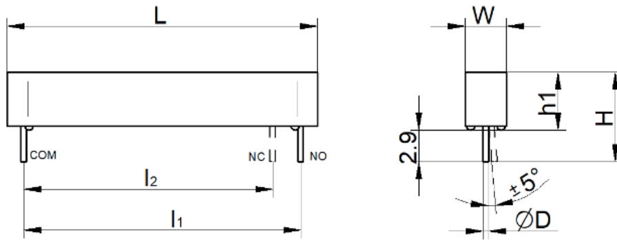
MRS06 Outline Drawing
